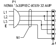
208-240 VAC 3 PHASE DELTA
